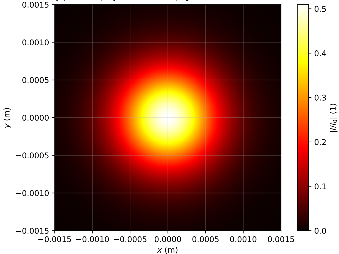
Intensity profile I(x, y, z = 3.821m)/I_0 , Pin=0.6Pcr, artificial time
